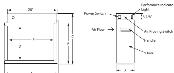
GA50A20, 22, 14 Dimensions
